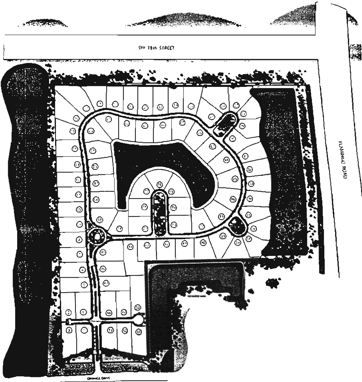
- Grove Creek Site Plan -
